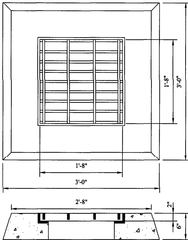
36" x 36" Precast Concrete Top
