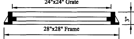
24"x24" Grate
