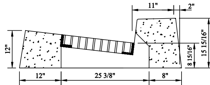
Plain Curb Type
