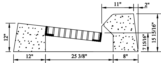
Bituminous Curb Type
