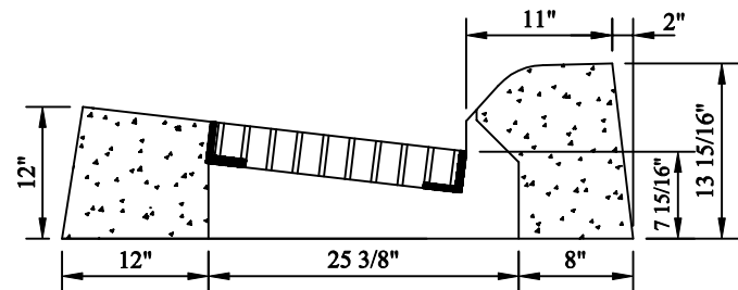
Park Curb Type
