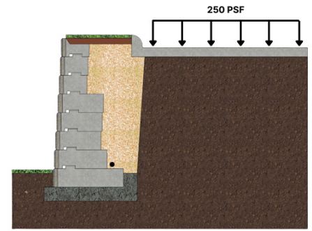
Flat Backslope - 250 PSF Surcharge
