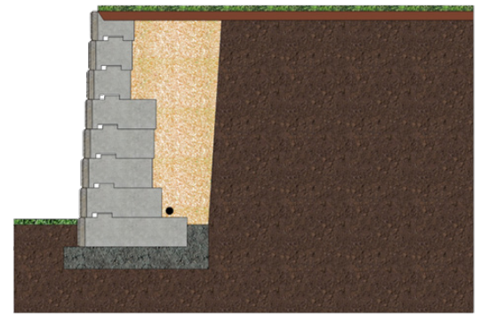
Level Backslope - No Surcharge
