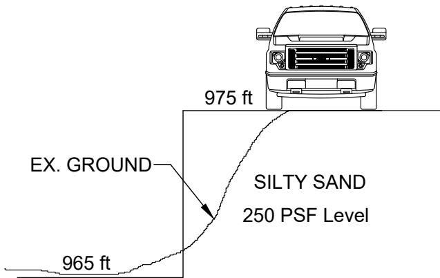
GEOMETRY AND SOILS
