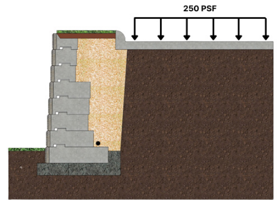
Flat Backslope - 250 PSF Surcharge
