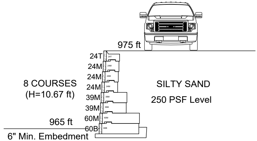
PRELIMINARY SECTION
