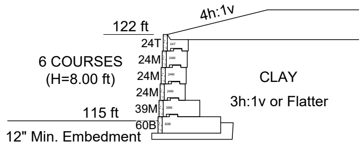
PRELIMINARY SECTION
