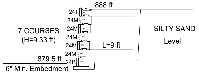
PRELIMINARY SECTION
